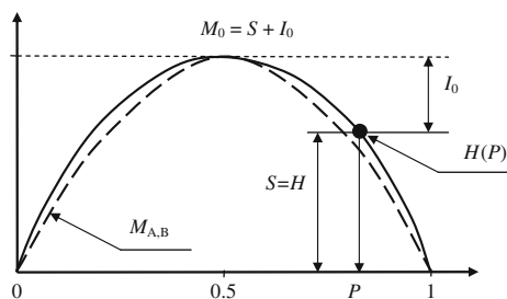
Fig. 4 Conservation of the overall entropic bond multiplicity M_0(P) = 1 bit in the 2-AO model of the chemical bond, combining the conditional-entropy (average noise, bond IT covalency) S(P) = H(P) and the mutual-information (information capacity, bond IT ionicity) I_0(P) = 1 - H(P) . In MO theory the direct bond-order of Wiberg [87] is represented by the (broken-line) parabola M_{A,B}(P) = 4P(1 - P) \equiv 4PQ
